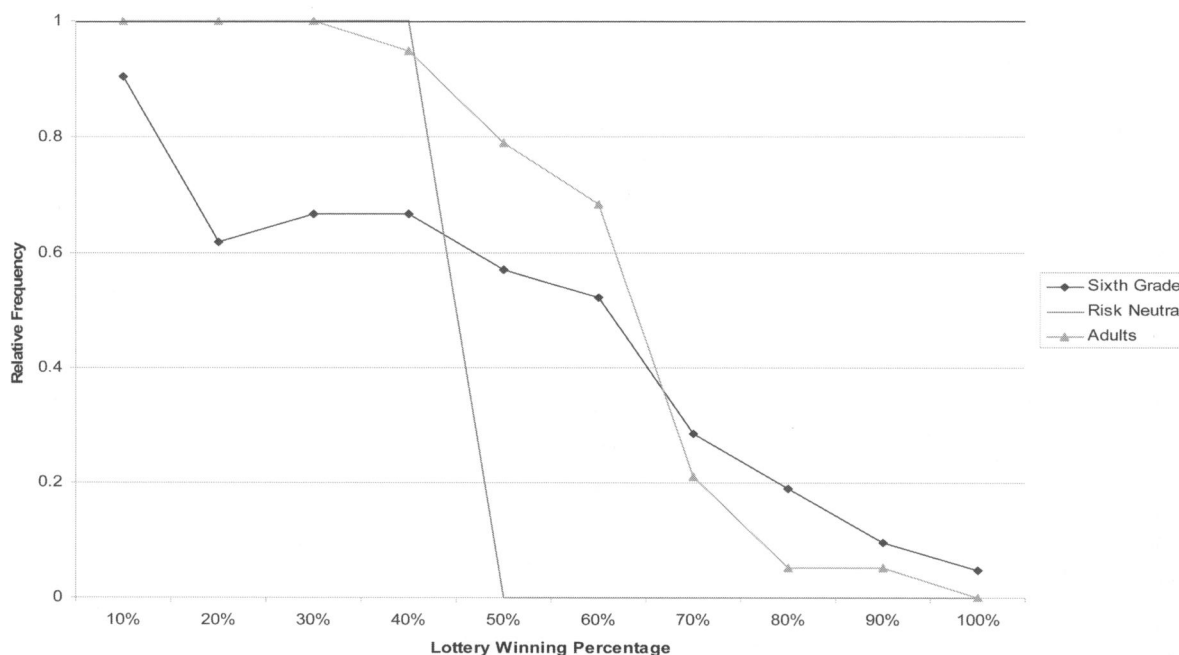
FIGURE 1. Percentage of Safe Lottery Choices.
