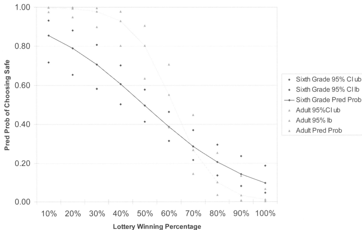
FIGURE 2. Probability of Choosing the Safe Lottery.
